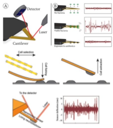
Figure 1. Setup of a nanomotion experiment. Depiction of typical bacteria or single cells analyses.
